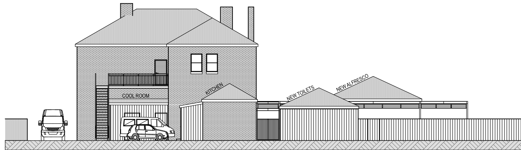
E3 REAR ELEVATION (EAST) 1:200
