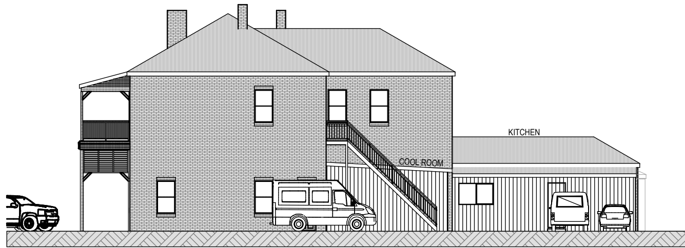
E2 SIDE ELEVATION (SOUTH) 1:200
