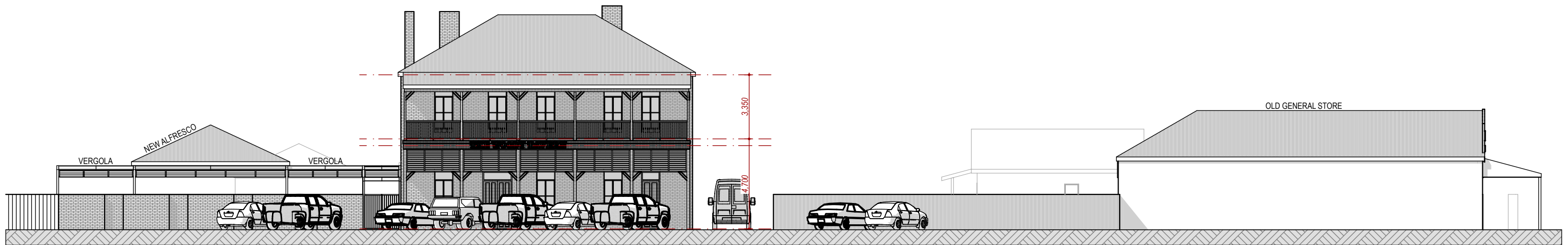
E1 FRONT ELEVATION / BURT ST (WEST) 1:200
